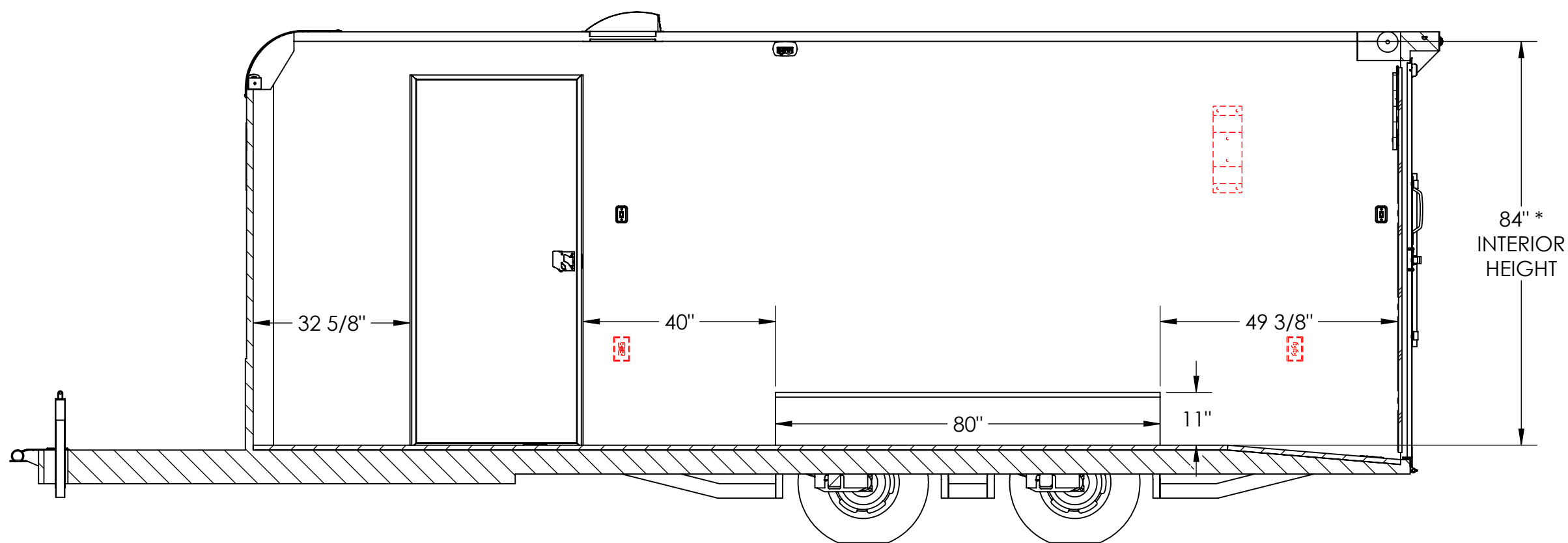
INTERIOR CURB SIDE SECTION B-B
