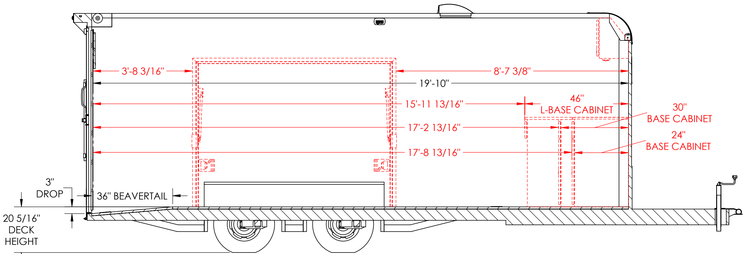
INTERIOR ROAD SIDE SECTION A-A
